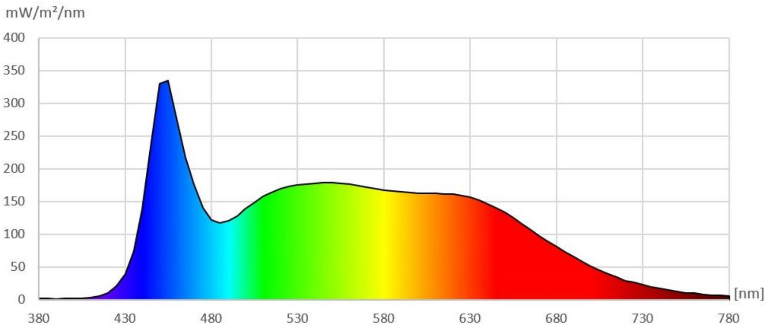
Wavelength White:
