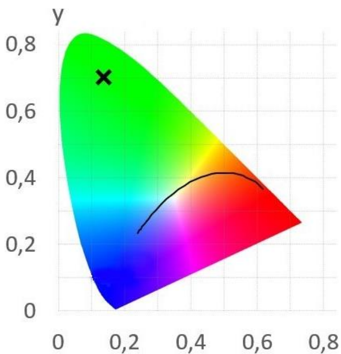
CIE1931 Green:
