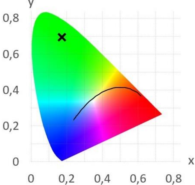
CIE1931 Green:
