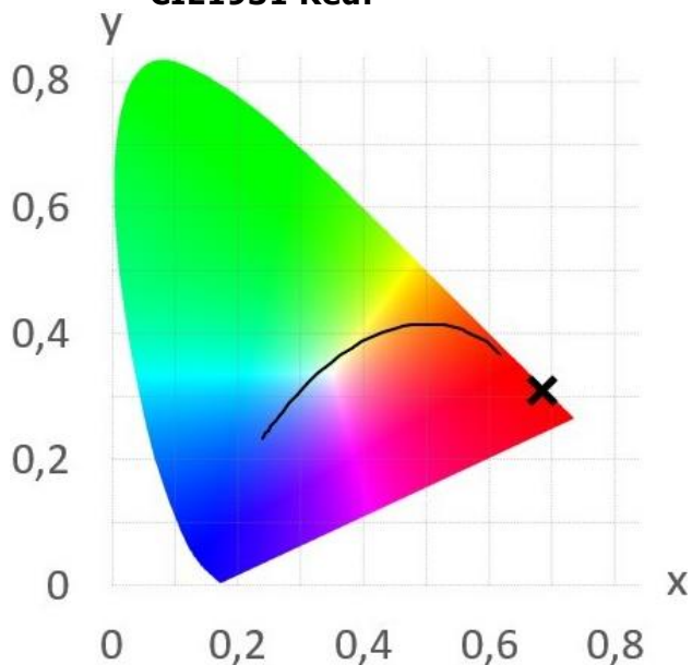
CIE1931 Red:
