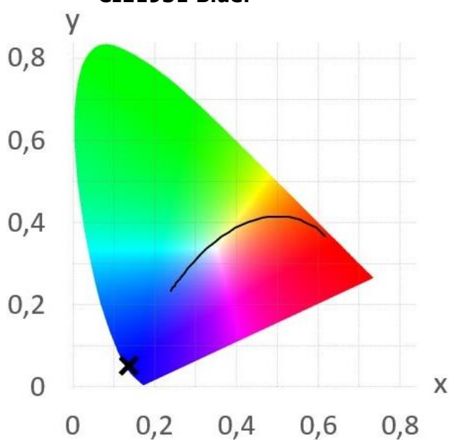
CIE1931 Blue:
