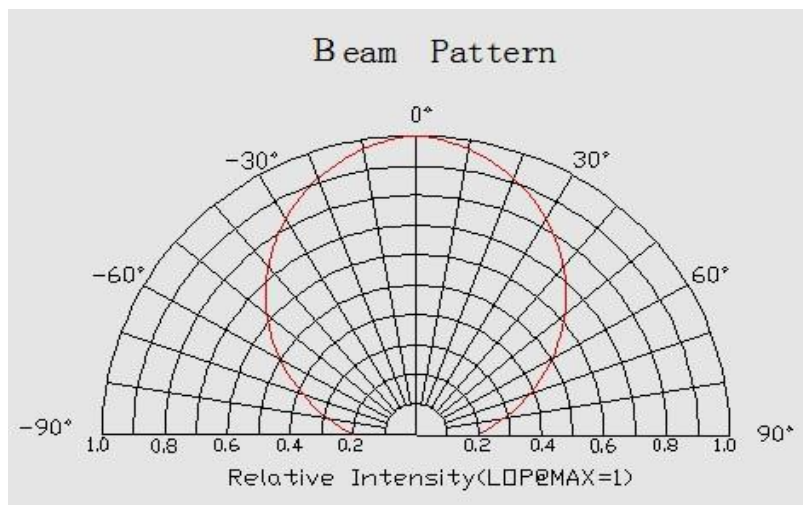
Optical Characteristics Curve:
