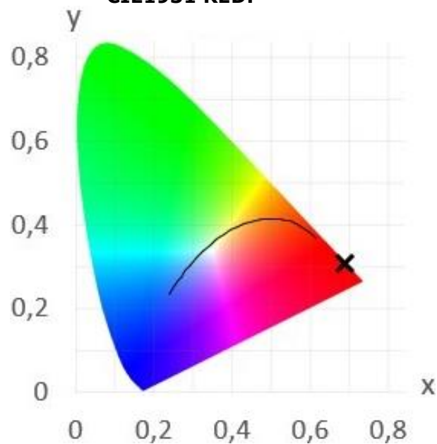
CIE1931 RED:
