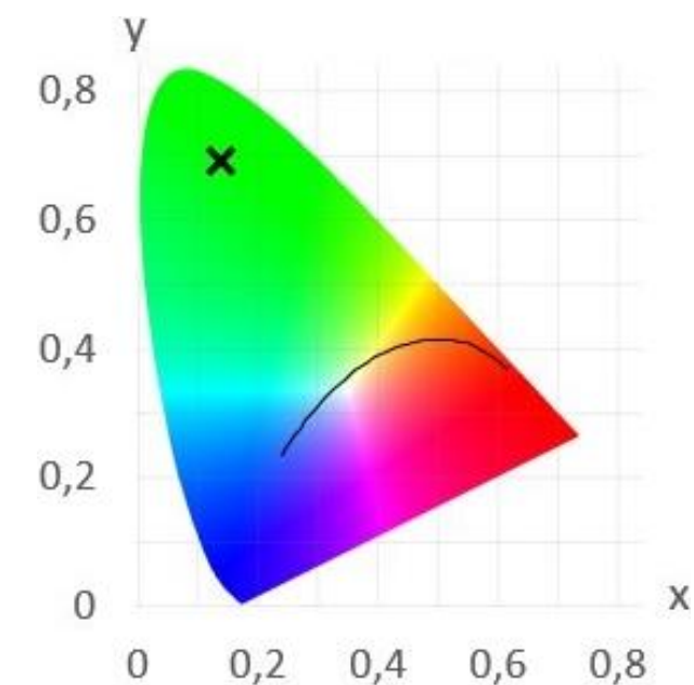
CIE1931 GREEN:
