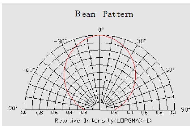
Optical Characteristics Curve:
