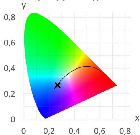
CIE1931 White:
