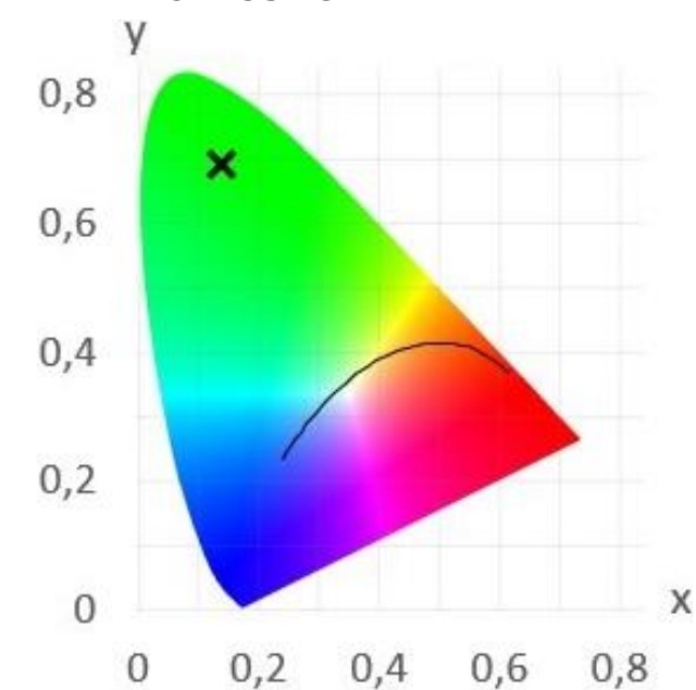
CIE1931 GREEN:
