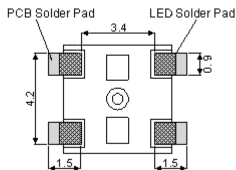
Solder Pad
